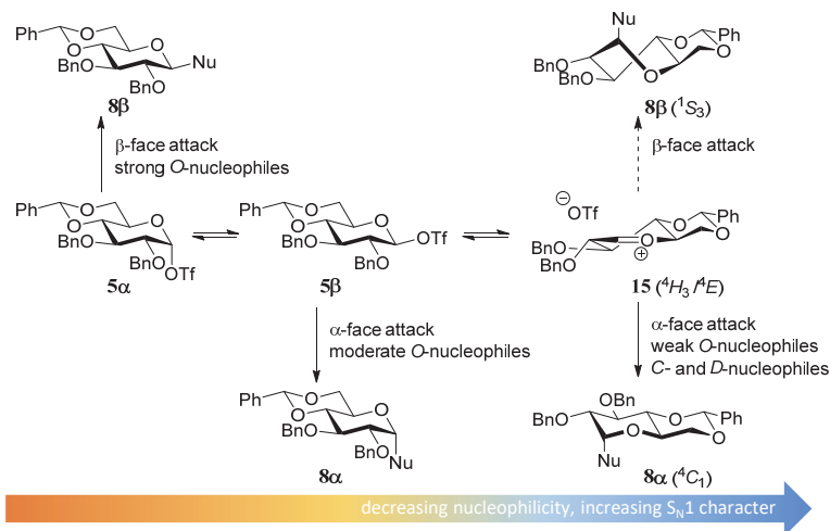
Figure 3. Mechanistic pathways to account for the selectivity in glycosylations of benzylidene glucose donors.
