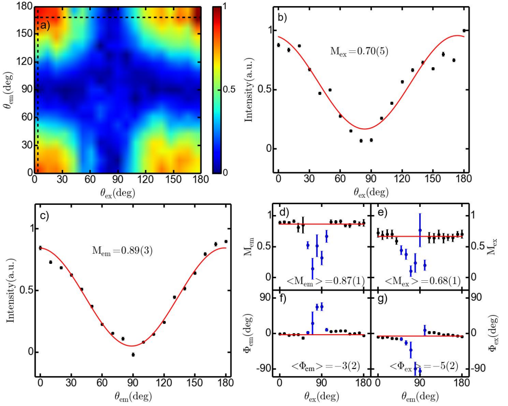
Figure 3.2: Polarization measurement of a single emitter. a) Intensity (color scale) of the emitter is presented as a function of excitation, \theta_{ex} , and emission polarization angles, \theta_{em} . Each of the cross-sections at constant excitation or emission polarization angle (vertical and horizontal) is fitted with the expected dependence for an ellipsoidal cluster (in the text) from which we obtain modulation depth, M , and phase, \Phi . b) Cross-section for \theta_{em} = 170^\circ gives M_{ex} = 0.70(5) . c) Cross-section for \theta_{ex} = 0^\circ gives M_{em} = 0.89(3) . d) Averaged emission modulation depth and e) averaged phase of the emitter are extracted from an error weighted linear fit (red line) of the data points from the cross-section fits. f) Averaged excitation modulation depth and g) averaged phase are found similarly as for d) and e). Cross-sections for which the intensity of the emitter is smaller than, or equally to the noise floor \epsilon_a , (see Figure 1b) are indicated as blue regions in (a). As explained in the text, data points extracted from those cross-sections (blue data points in 2d-g) are not reliable and are therefore excluded in determining the average modulation depth \langle M \rangle .
