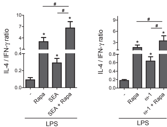
Figure S3. Co-stimulation with rapamycin and SEA or omega-1 primes a stronger Th2 response than stimulation with rapamycin, SEA or omega-1 alone. moDCs were either pulsed with SEA or omega-1 in combination with LPS, and / or incubated for 90 minutes with rapamycin, or its vehicle DMSO prior to stimulation. T cell responses were analysed as described for Supplementary figure 2. Bars represent mean values + s.e.m.; *,# P < 0.05 ; for significant differences with the LPS control (*) or between test conditions (#) based on one-sided Wilcoxon signed rank testing. ω-1, omega-1; Rapa, rapamycin.
