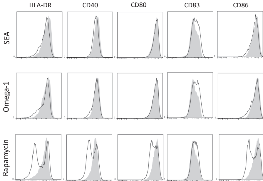
Figure S1. Rapamycin lowers LPS-induced DC maturation. moDCs were either pulsed with SEA or omega-1 in the presence of LPS, or incubated for 90 minutes with rapamycin or its vehicle DMSO prior to LPS stimulation. After 48 hours, expression of maturation markers was analyzed by flow cytometry. Representative histograms from 1 out of 9 independent experiments are shown. Filled histograms represent control conditions (either LPS or LPS + DMSO).
