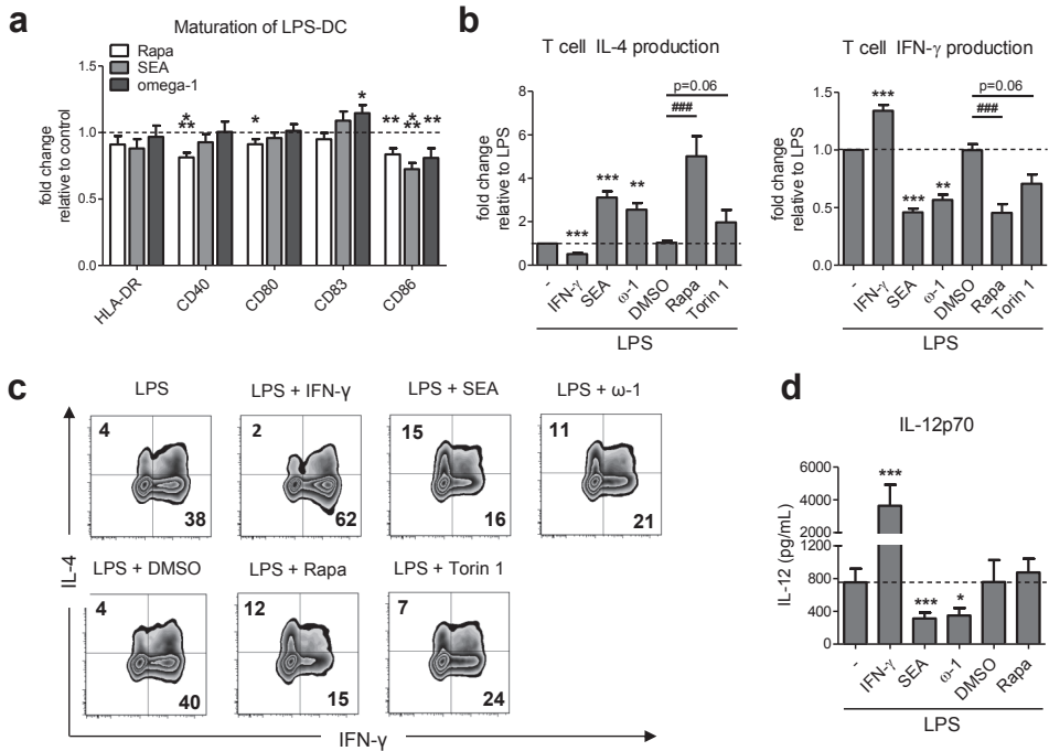
Figure 1. Rapamycin lowers DC maturation and primes for Th2 responses without affecting DC IL-12 production. (a) moDCs were either pulsed with SEA or omega-1 in the presence of LPS, or incubated for 90 min with rapamycin or its vehicle dimethyl sulfoxide (DMSO) prior to LPS stimulation. After 48 h, expression of maturation markers was analyzed by flow cytometry. The expression levels, based on the geometric mean fluorescence of at least nine independent experiments, are shown relative to the moDCs stimulated with LPS or LPS + DMSO alone, which were set to 1 for each marker (dashed line). (b) moDCs were either pulsed with SEA or omega-1 in combination with LPS, or incubated for 90 min with rapamycin, Torin1 or their vehicle DMSO prior to LPS stimulation. After 48 h of stimulation, moDCs were cultured with allogeneic naive CD4 + T cells for 11 days. Intracellular IL-4 and IFN- \gamma were analyzed by flow cytometry after a 6-h stimulation with phorbol myristate acetate and ionomycin. IFN- \gamma -stimulated moDCs were taken along as a Th1-inducing control. The percentages of T cells uniquely positive for either IL-4 or IFN- \gamma are expressed relative to the LPS condition. Data represent at least four independent experiments. (c) Representative FACS plots from one out of the four independent experiments are shown for conditions described for Figure 1b. (d) Following stimulation as described for Figure 1a, conditioned moDCs were co-cultured with a CD40L-expressing cell line. Supernatants were collected after 24 h and IL-12p70 concentrations were determined by ELISA. IFN- \gamma -stimulated moDCs were taken along as an IL-12 inducing control. Bars represent mean values + s.e.m.; * P <0.05; ** P <0.01; ***, ### P <0.001 for significant differences with the control (*; either LPS or LPS + DMSO) or between test conditions (#), based on one-sided Wilcoxon-signed rank testing. \omega -1, omega-1; Rapa, rapamycin.
