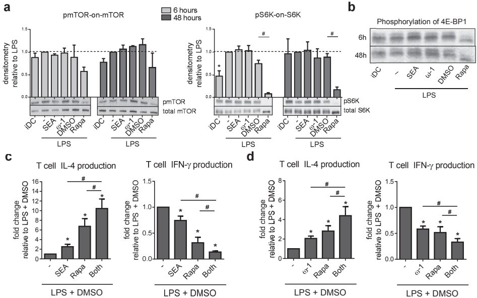
Figure 2. Unlike rapamycin, SEA and omega-1 do not affect the mTOR pathway to condition DCs for Th2 priming. MoDCs were stimulated as described in the legend of Figure 1. (a,b) moDC lysates were collected after 6 and 48 h of stimulation. Proteins were visualized by western blotting using antibodies against S6K and S6K phosphorylation at Thr421, and mTOR and mTOR phosphorylation at Ser2448. Western blot results were quantified using ImageJ software. The pS6K-on-S6K and pmTOR-on-mTOR ratios were calculated relative to the LPS condition. Representative blots from one out of five (6 h) or four (48 h) independent experiments are shown. (b) moDC lysates were collected after 6 and 48 h of stimulation. 4E-BP1 phosphorylation at Thr37/46 was assessed by western blotting. (c,d) moDCs stimulated for 48 h were cultured with allogeneic naive CD4 + T cells for 11 days and T-cell cytokine production was analyzed as described in the legend of Figure 1. Data represent at least five independent experiments. Bars represent mean values \pm s.e.m.; *, #P<0.05 for significant differences with the control (*, either LPS or LPS + DMSO) or between test conditions (#) based on one-sided Wilcoxon-signed rank testing. iDC, immature (nonstimulated) moDC; \omega -1, omega-1; Rapa, rapamycin; Both, rapamycin and SEA or omega-1.
