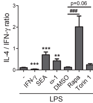
Figure S2. Rapamycin primes DCs for Th2 responses. moDCs were either pulsed with SEA or omega-1 in combination with LPS, or incubated for 90 minutes with rapamycin, Torin1 or their vehicle DMSO prior to LPS stimulation. After 48 hours of stimulation, moDCs were cultured with allogeneic naive CD4 + T cells for 11 days. Intracellular IL-4 and IFN-γ were analyzed by flow cytometry after 6h stimulation with PMA and ionomycin. IFN-γ-stimulated moDCs were taken along as a Th1-inducing control. The ratio of T cells uniquely positive for either IL-4 or IFN-γ was calculated. Data represent at least 4 independent experiments. Bars represent mean values + s.e.m.; ** P < 0.01 ; *** P < 0.001 for significant differences with the LPS control (*) or between test conditions (#) based on one-sided Wilcoxon signed rank testing. ω-1, omega-1; Rapa, rapamycin.
